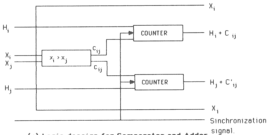
(c) Logic design for Comparator and Adder
